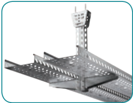
Taşıyıcı Destek Sistemleri / DS Series Carrier Support Systems
