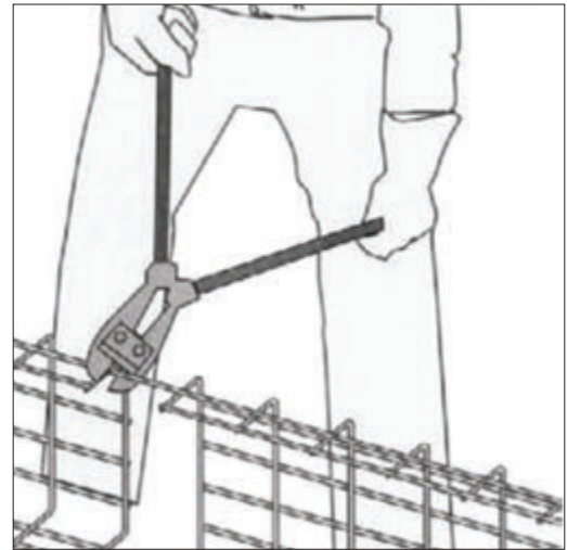
Yan Kenar Alt Telleri Kes Side Edge Lower Wires Cut
