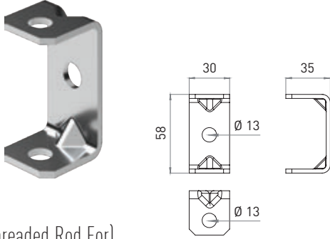
Tijli Tavan Tespit Ceiling Installation (Threaded Rod For)
