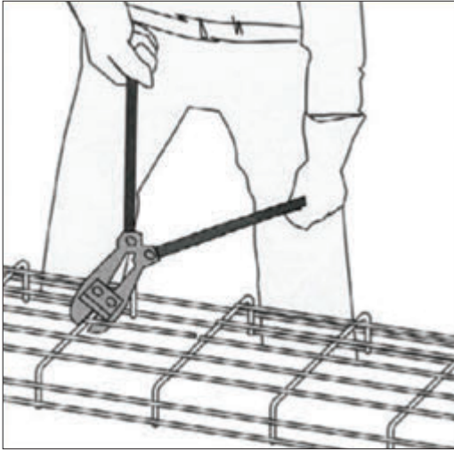
Alt Telleri Kes Sub Wires Cut
