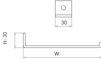
Delikli L Askı Ayağı Perforated L Hanging Supports
