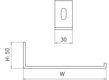
Delikli L Askı Ayağı Perforated L Hanging Supports
